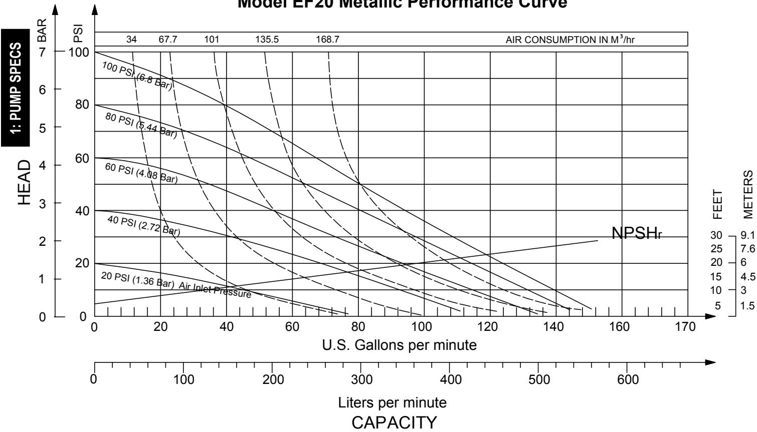
Model EF20 Metallic Performance Curve
