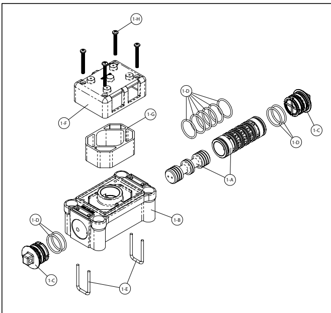
Air End Section Assembly
