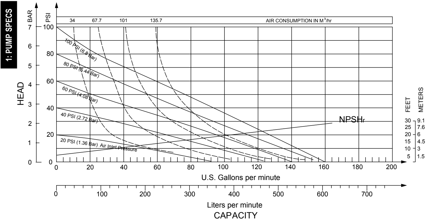
Model EF20 Non-Metallic Performance Curve
