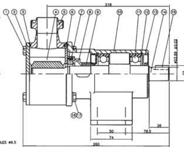
HALF SECTION X - X
