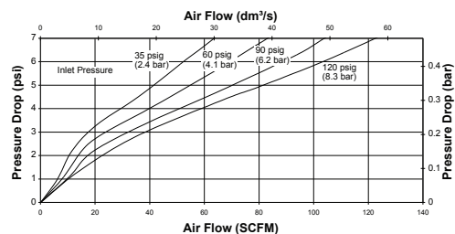
3/8" 1500 SERIES LUBRICATOR
