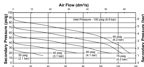
3/8" 1500 SERIES FILTER/REGULATOR
