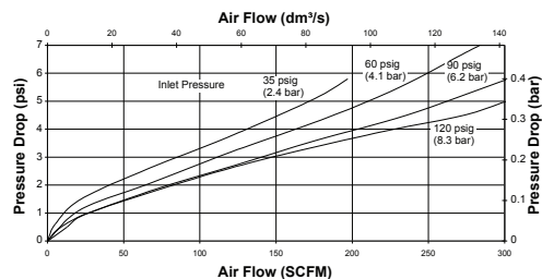
3/4" 3000 SERIES LUBRICATOR
