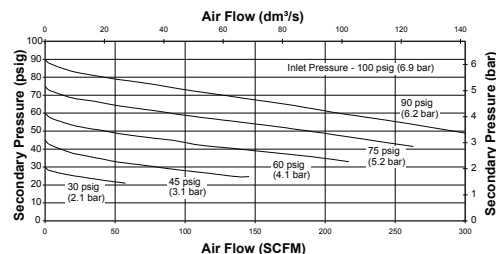
3/4" 3000 SERIES FILTER/REGULATOR
