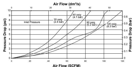
3/8" 1500 SERIES FILTER
