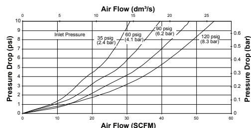
1/4" 1000 SERIES FILTER
