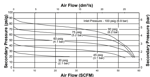
1/4" 1000 SERIES FILTER/REGULATOR
