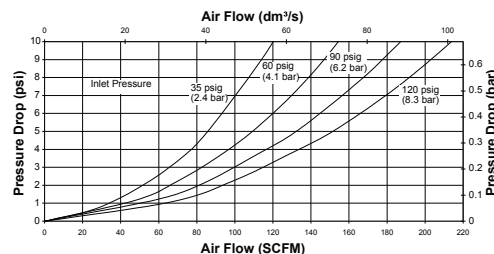
1/2" 2000 SERIES FILTER
