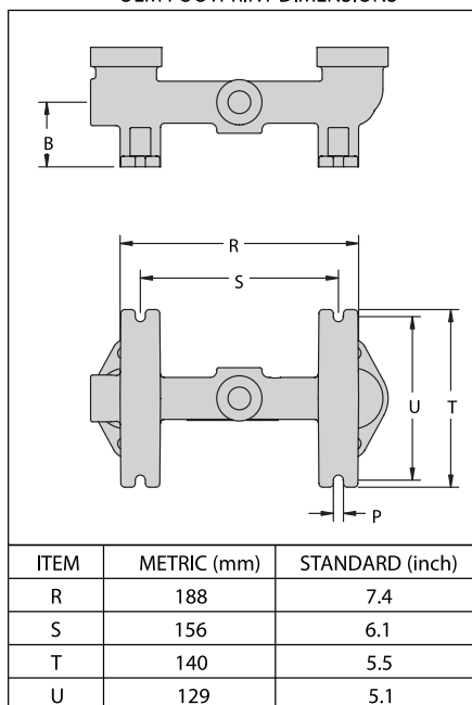
OEM FOOTPRINT DIMENSIONS
