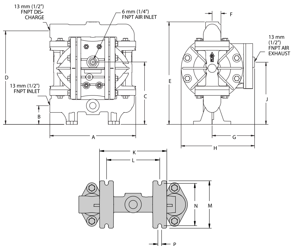
OEM FOOTPRINT DIMENSIONS
